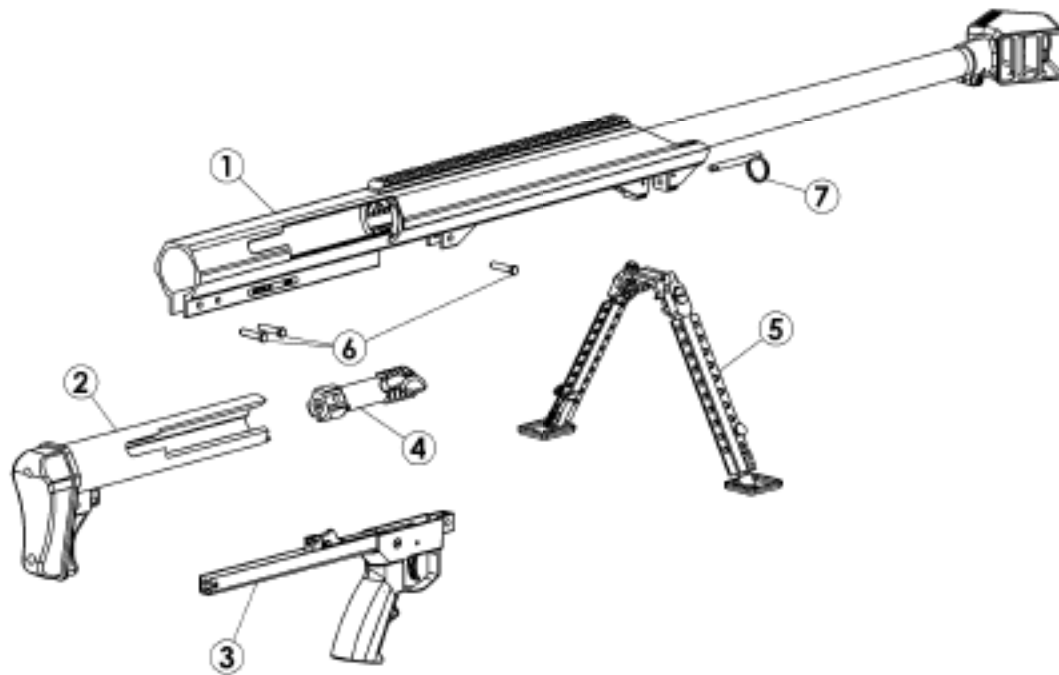
Figure 6. Major components.
