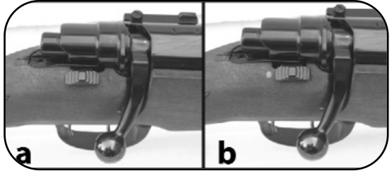
Safety in M70 and M85 in "ON" position.
