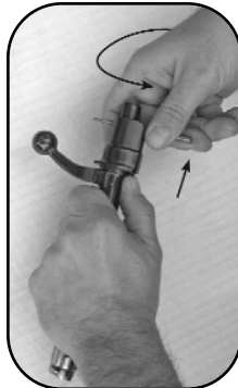
Separation of hammer mechanism.
